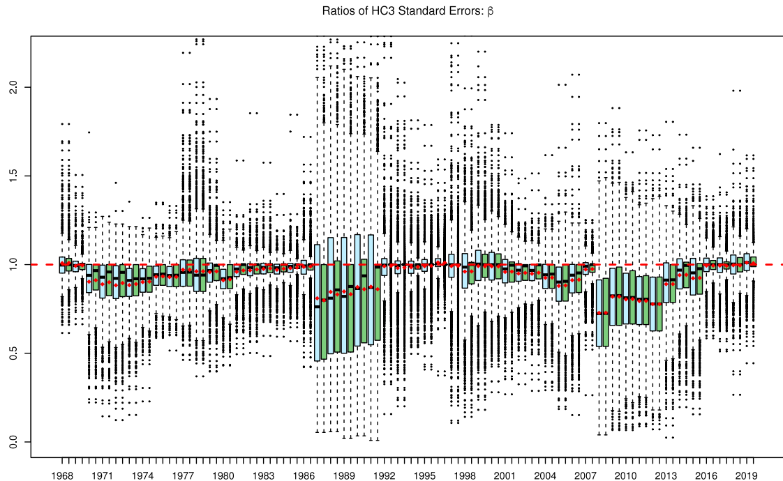
Fig. 3. CAPM boxplots for the two ratios defined in (4.1) over 52 years for the parameter of interest \beta := \beta_2 . For any year, we plot first the WLS/OLS boxplots in blue, followed by the ALS/OLS boxplots in green. In each box, the bar indicates the median ratio whereas the diamond-shaped symbol indicates the average ratio. (For interpretation of the references to color in this figure legend, the reader is referred to the web version of this article.)
